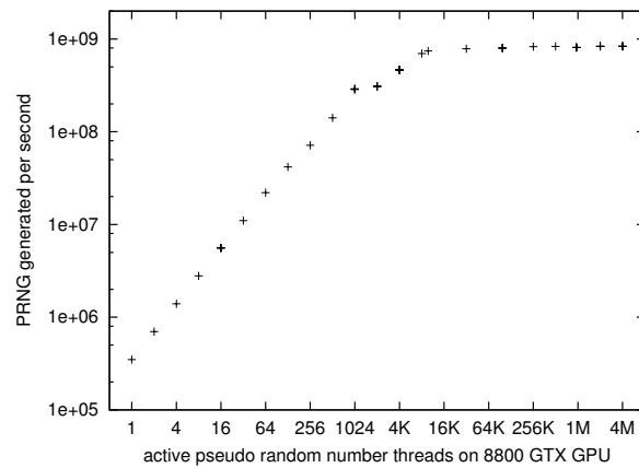
Fig. 7. Park-Miller random numbers per second (excluding host-GPU transfer time) on nVidia 8800 GTX. In the test environment the rate depends upon how effectively the 128 parallel stream processors can be used. Only when there are more than 8192 separate threads do the 128 stream processors effectively saturate.
